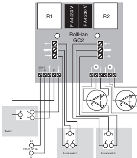
Fig. 2. GC2 group control connection diagram
