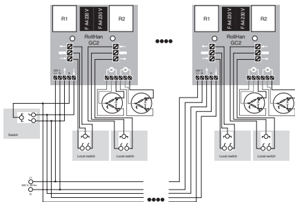
Fig. 3. GC2 block connection diagram
